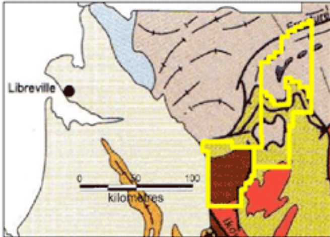
Geological setting of Dome's properties in Gabon (Pink = Archaean; Green/Brown = Deformed Proterozoic)
